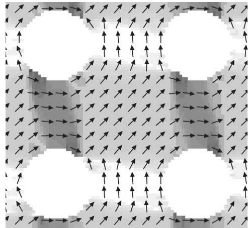
Fig. 22. A micromagnetic simulation of the spin configuration of magnetic induction in a bit constrained at the corners by four antidots (holes). Adapted from Ref. [130].
