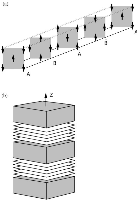
Fig. 17. (a) Schematic diagram illustrating the Type-III antiferromagnetic structure. (b) Schematic diagram showing how the antiferromagnetic planes of the Type-III structure are arranged in a superlattice.
