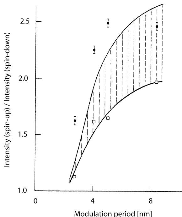
Fig. 8. Measured ratio of spin-up neutron intensity to spin-down intensity (•) plotted as a function of modulation period in the Ni/Mo superlattice. The experimental measurements are consistently larger than those calculated for a wide variety of model structures in which the magnetic roughness was constrained to be the same as the chemical roughness (as determined from X-ray scattering), indicating that the magnetic Ni/Mo interface is smoother than the chemical Ni/Mo interface. Adapted from Ref. [86].
