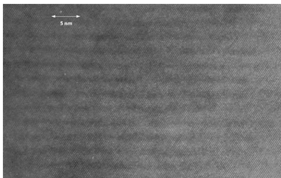
Fig. 20. A TEM micrograph of a (\text{MnSb}) \times_1 (\text{GaSb}) \times_6 digital superlattice (“digital alloy”) grown by atomic layer epitaxy. The Mn-containing “digital” layers are much thinner than the image indicates, because TEM is significantly more sensitive to the strain produced by the inserted atomic species than to its atomic number. Adapted from Ref. [295].
